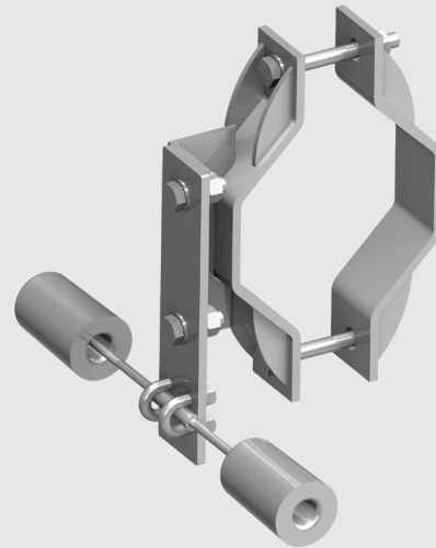
Vibration Dampers
