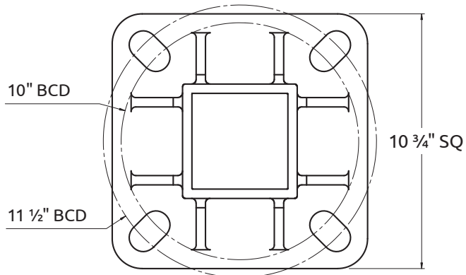
NSSA Type A2 (1" x 24" Anchor Bolts) Select A2 Base Plate in Options column on reverse page
