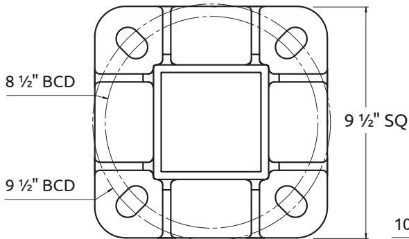
NSSA Type A ( \frac{3}{4} " x 24" Anchor Bolts) Default Base Plate Option
