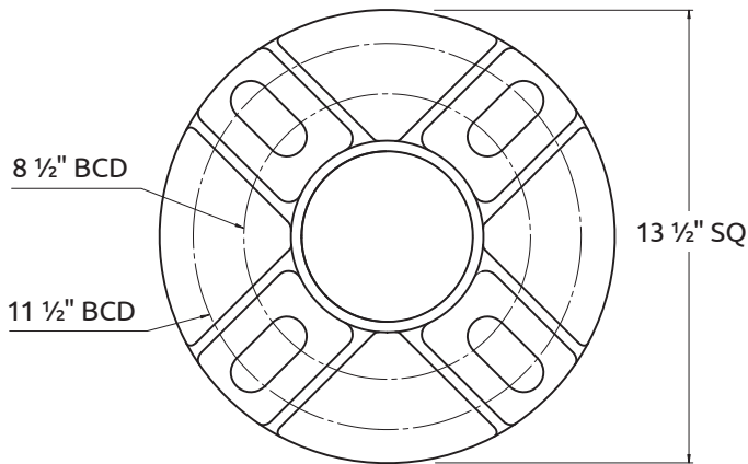
NSRA Type B (1" x 36" Anchor Bolts)
