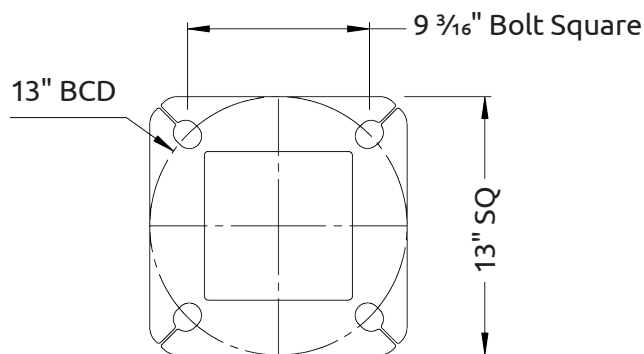
NSQT Type B (1" Anchor Bolts)
