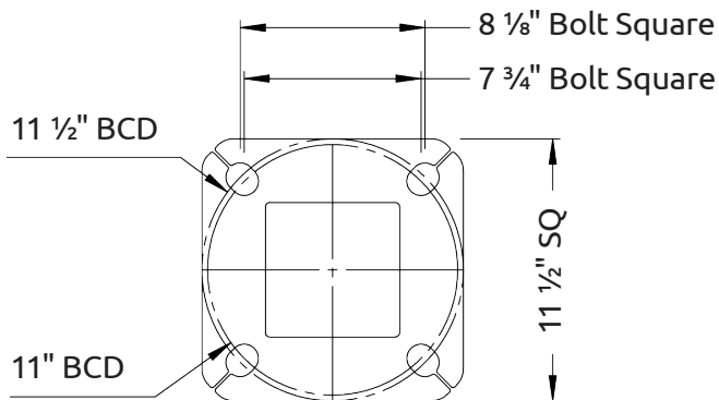
NSQT Type A (1" Anchor Bolts)
