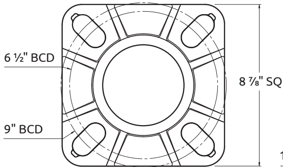
NSRA Type A (3/4" x 24" or 1" x 24" Anchor Bolts) Default Base Plate Option
