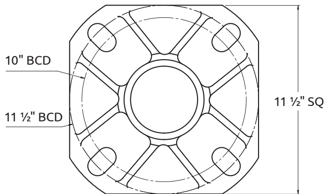
NSRA Type A2 (1" x 24" Anchor Bolts) Select A2 Base Plate in Options column on reverse page
