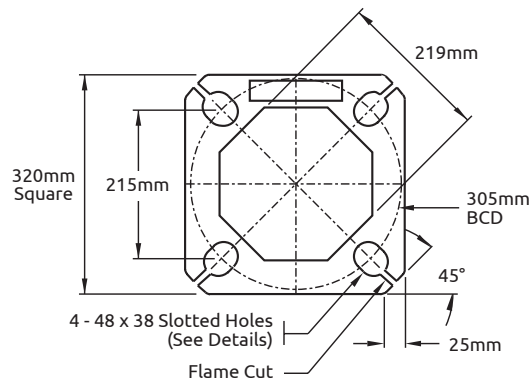
TYPE 2 BASE PLATE - PLAN VIEW For 11.0m Shaft
