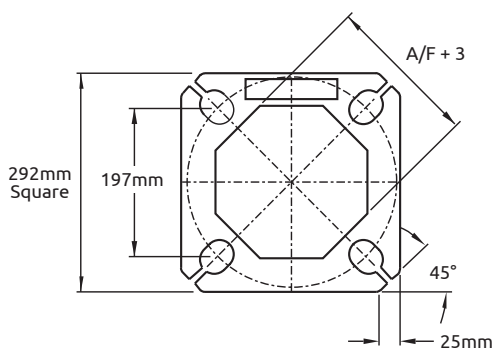
TYPE 2 BASE PLATE - PLAN VIEW
