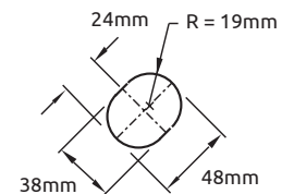
SLOTTED HOLE DETAIL
